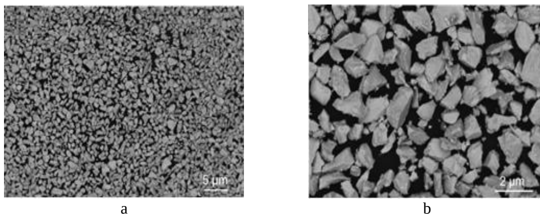
Figure 1 – Structure of the T15K6 alloy: a) with the addition of WC nanopowder; b) with the addition of WC nanopowder with deposited cobalt
